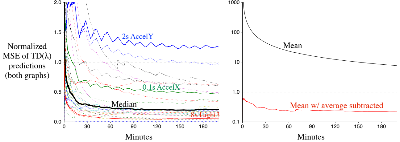
Fig. 8. Learning curves for the 212 predictions whose pseudo reward is a sensor reading. The median and several representative learning curves are shown on a linear scale on the left, and the mean learning curve is shown on a logarithmic scale on the right. The mean curve is high because of a minority of the sensors whose absolute values are high and whose variance is low. If the experiment is rerun using pseudo rewards with their average value subtracted out, then the mean performance is greatly improved, as shown on the right, explaining 78% of the variance in the ideal prediction by the end of the data set.
