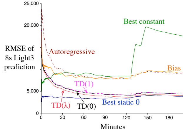
Fig. 7. Learning curves for 8-second Light3 predictions made by various algorithms over the full data set. Each point is the RMSE of the prediction of the algorithm up to that time. Most algorithms use only the data available up to that time, but the best-static- \theta and best-constant algorithms use knowledge of the whole data set. The errors of all algorithms increased at about 130 and 150 minutes because the motors overheated and shutdown at those times while the robot was passing near the light, causing an unusual pattern of sensor readings. In spite of the unusual events, the RMSE of TD(\lambda) still approached that of the best static weight vector. See text for the other algorithms.
