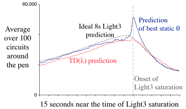
Fig. 5. Light3 predictions (like those in the lower portion of Figure 4) averaged over 100 circuits around the pen and aligned at the onset of Light3 saturation.
